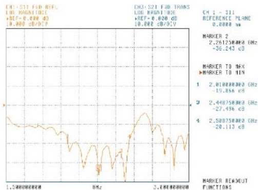
Return Loss
