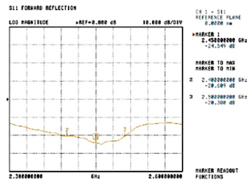
Return Loss
