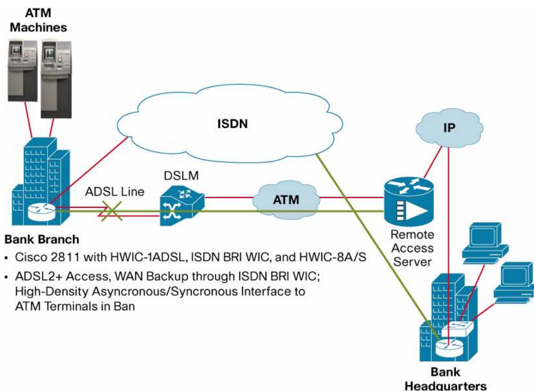
Figure 5. Banking Application
